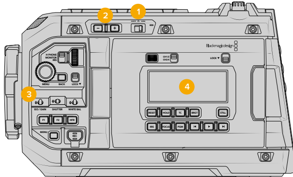
URSA Cine with the foldout touchscreen closed
