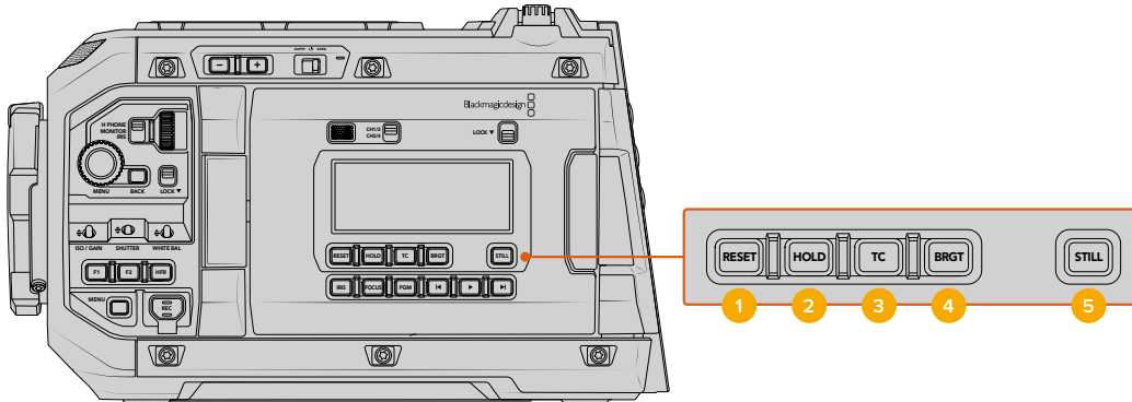
URSA Cine status LCD controls
