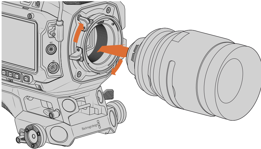
Attaching and removing a PL lens
