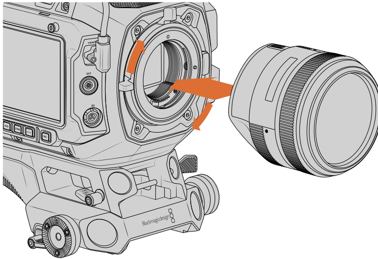
Attaching and removing an EF mount lens
